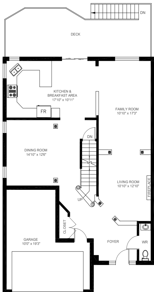
MAIN FLOOR (1,061 sq.ft.) Ceiling Height: 9'
