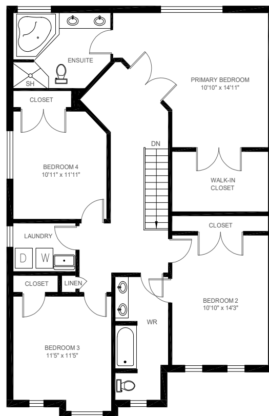
SECOND FLOOR (1,339 sq.ft.) Ceiling Height: 8'
