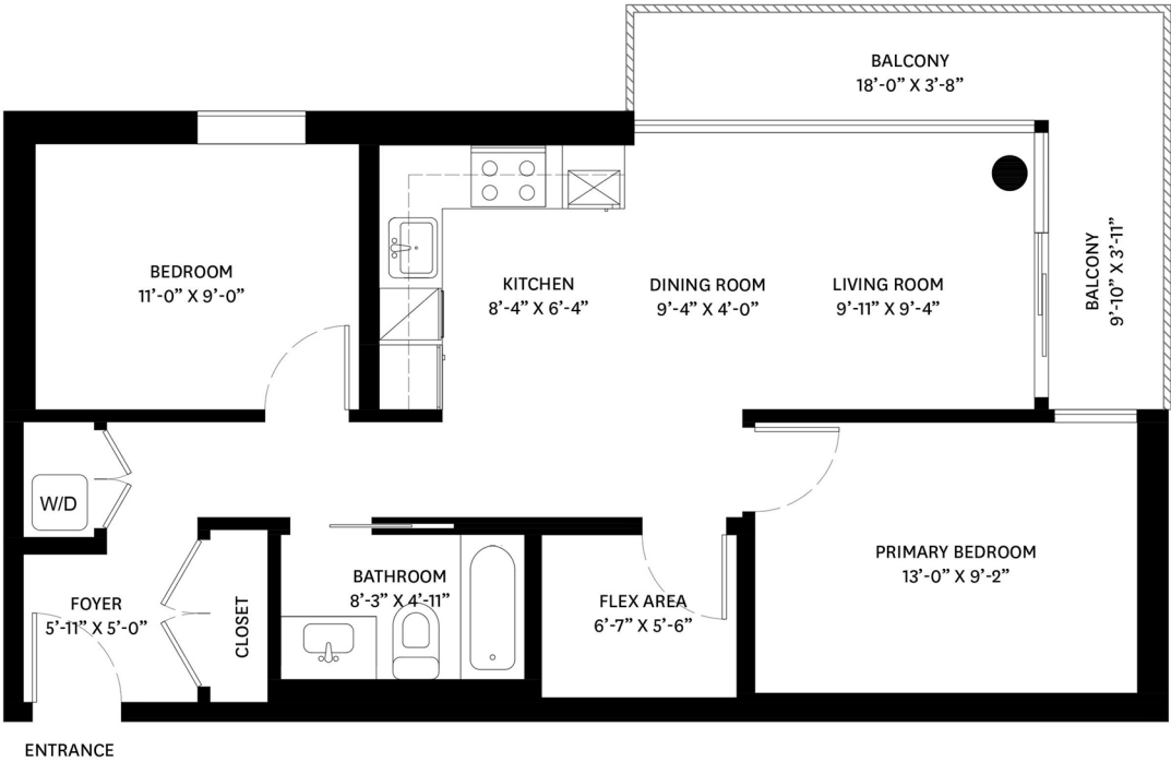
MAIN FLOOR PLAN Ceiling Height: 8'-6"
