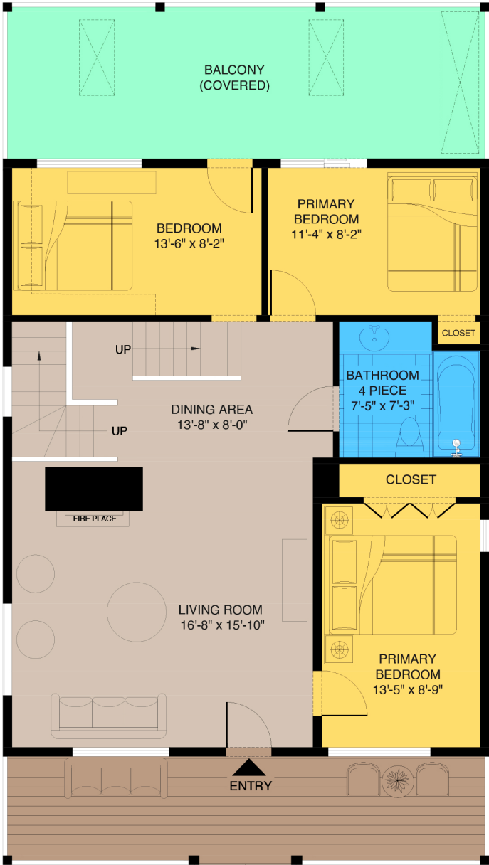
CEILING HEIGHT 7'-4" - 8'-0" MAIN FLOOR 832 SQ FT
