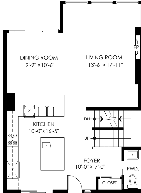
Lower Floor Plan Floor Area: 755 sq.ft. Ceiling Height: 8'
