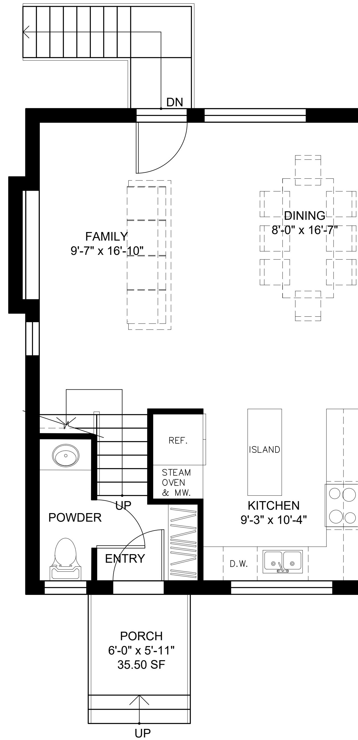
MAIN FLOOR PLAN
