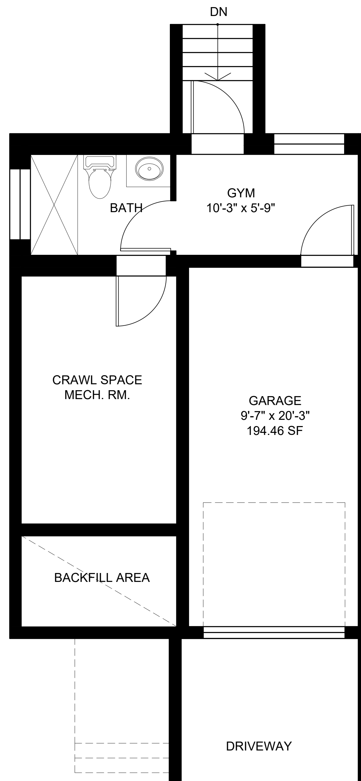
BASEMENT PLAN
