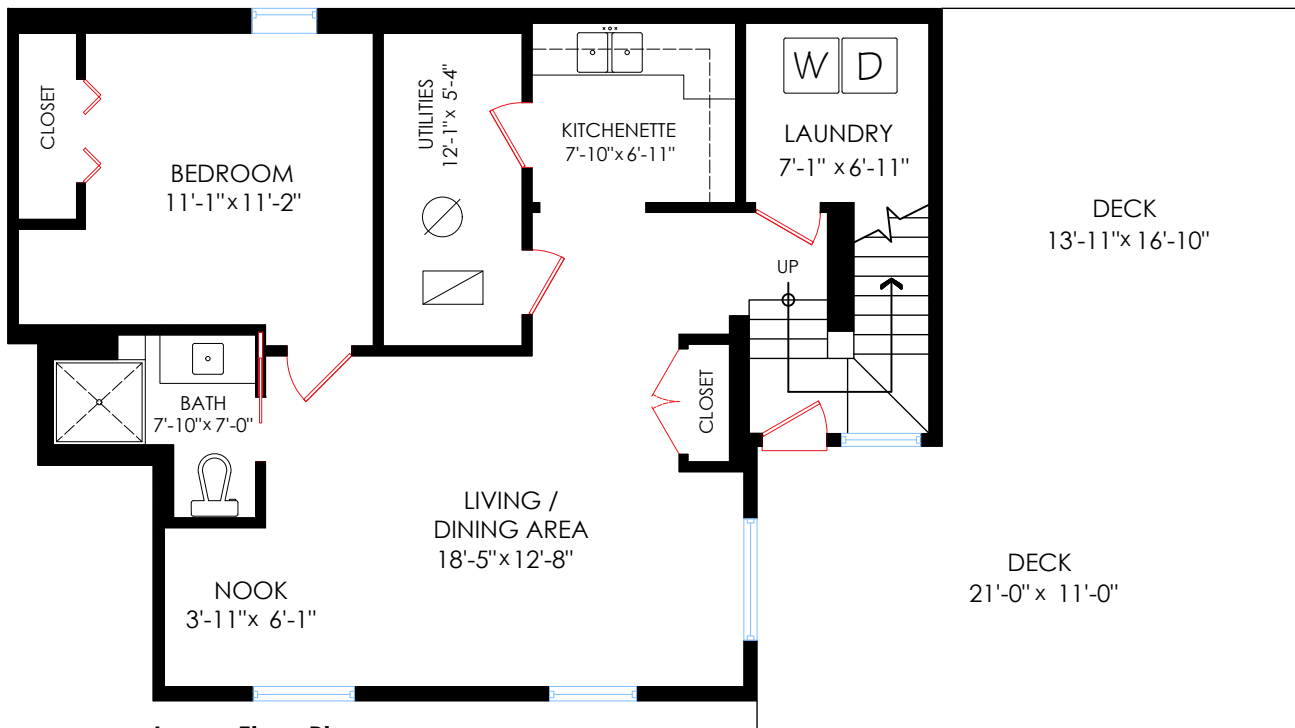
Lower Floor Plan Floor Area: 833 sq.ft. Ceiling Height: 8'
