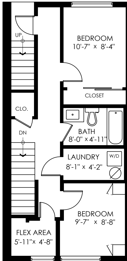
Upper Floor: 518 Sq.Ft. Ceiling Height: 7'-11"
