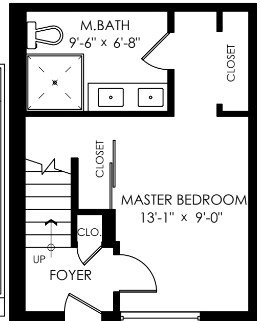
Lower Floor: 351 Sq.Ft. Ceiling Height: 7'-11"
