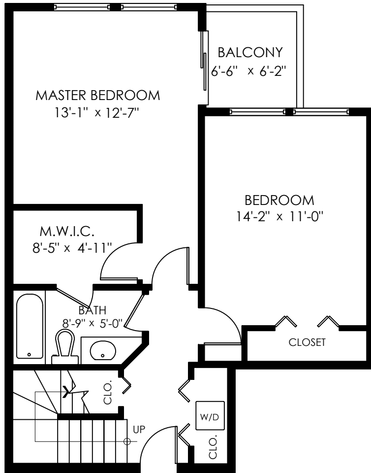
Lower Floor: 645 Sq.Ft. Ceiling Height: 8'-0"
