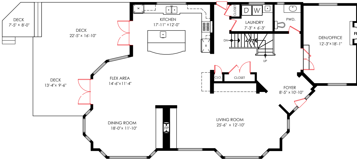
Main Floor Plan Floor Area: 1840 sq.ft. Ceiling Height: 8'-5"
