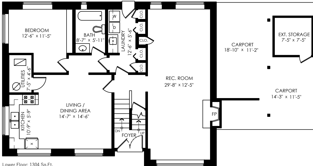
Lower Floor: 1304 Sq.Ft. Ceiling Height: 8'-3"
