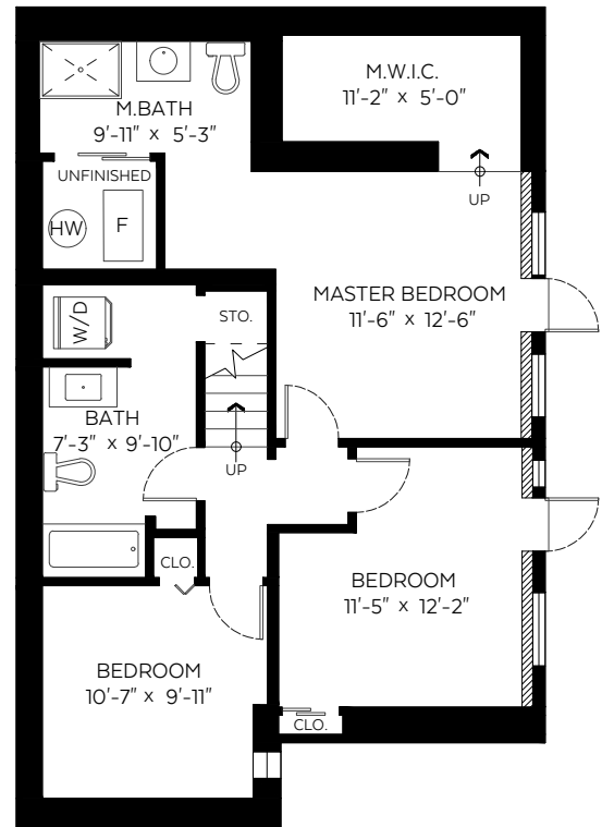
Lower Floor Plan Floor Area: 902 sq.ft.
