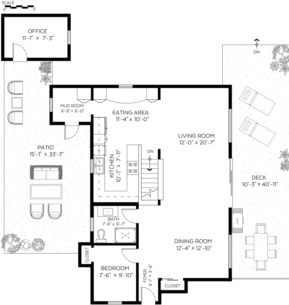
Main Floor Plan Floor Area: 970 sq.ft
