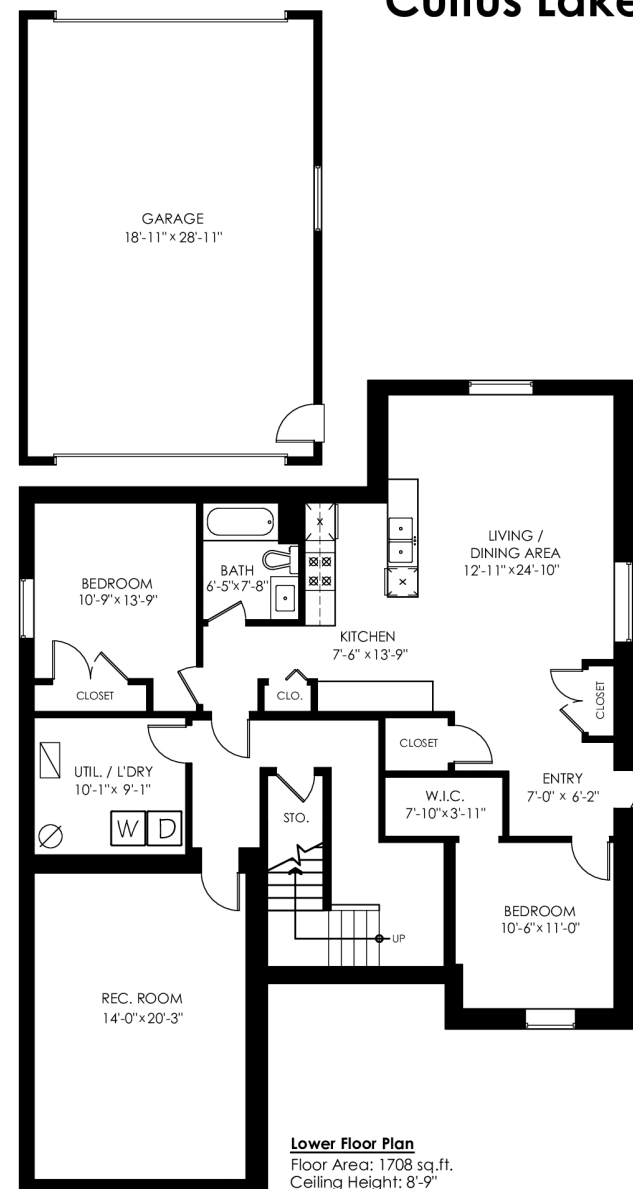
Main Floor Plan Floor Area: 1360 sq.ft. Ceiling Height: 8'-11"
