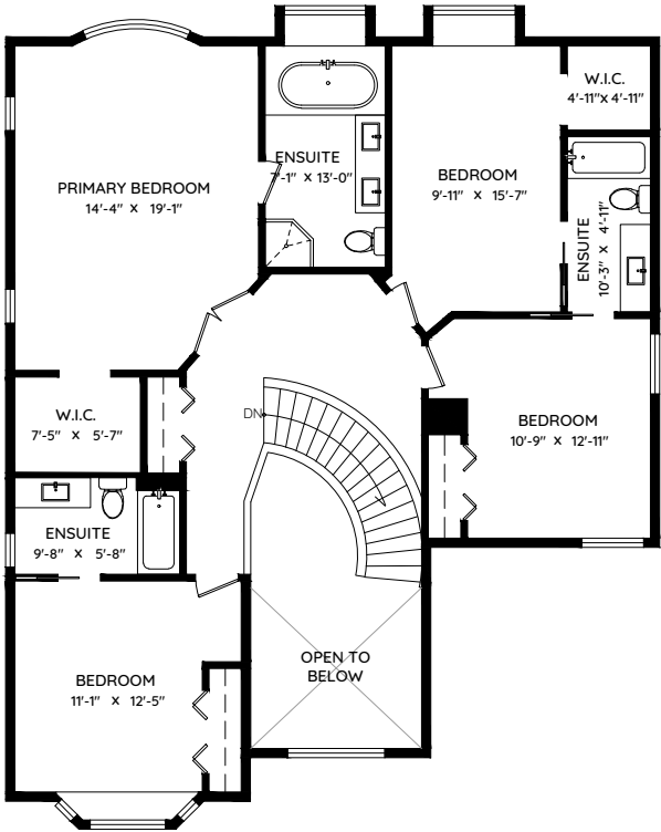
UPPER FLOOR 1,357 SQ.FT. CH: 8'-0"
