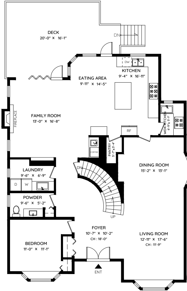
MAIN FLOOR 1,695 SQ.FT. CH: 9'-0"
