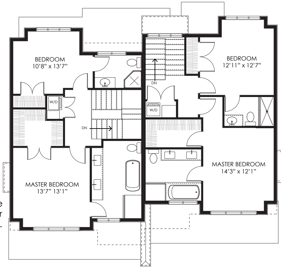
2070 Fulton Avenue Upper Floor 730 sq. ft.
