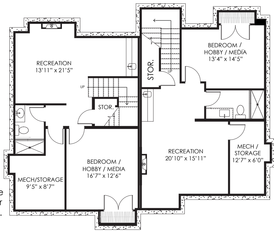
2070 Fulton Avenue Lower Floor 782 sq. ft.
