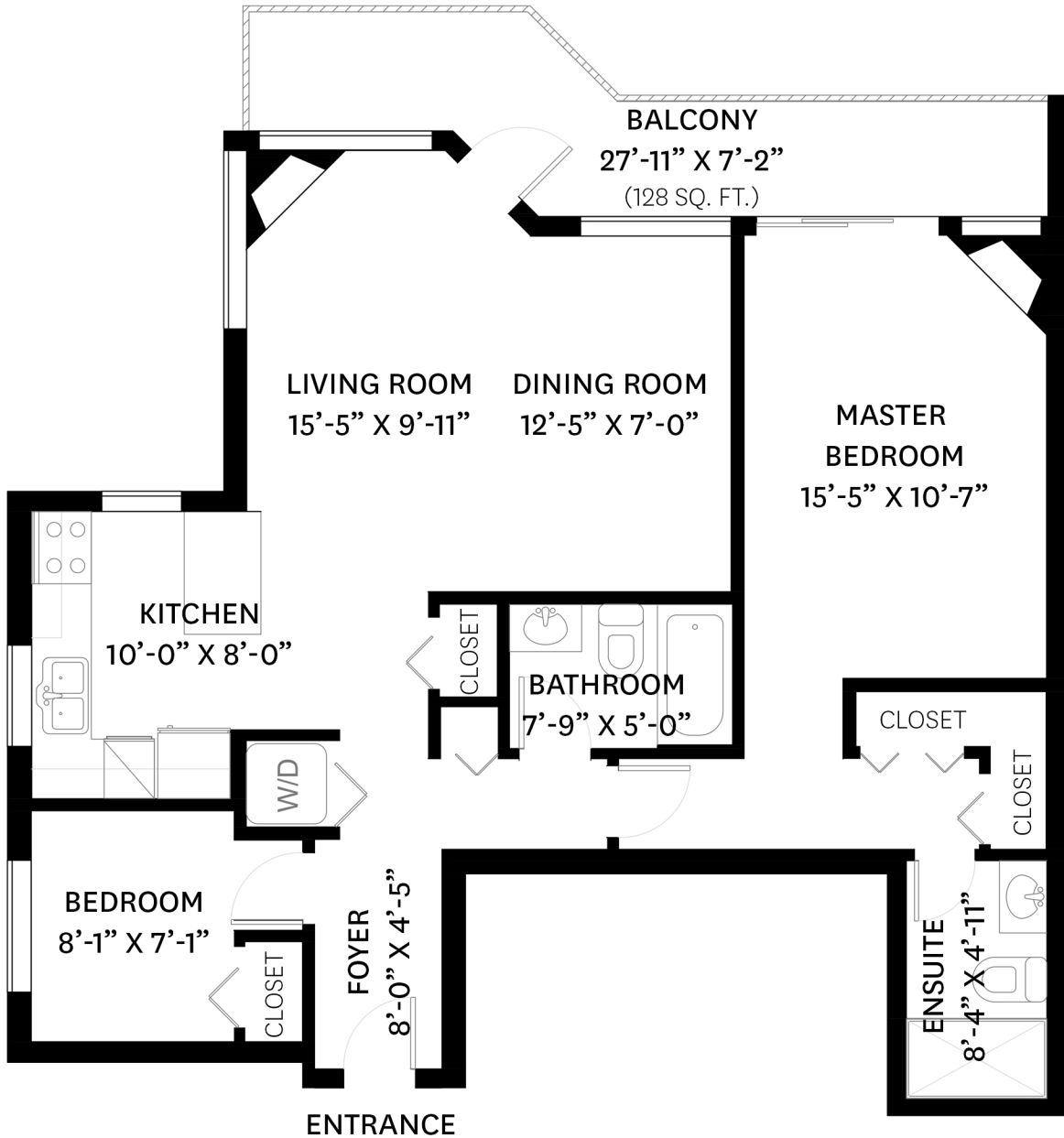
MAIN FLOOR PLAN Ceiling Height: 8'-0"
