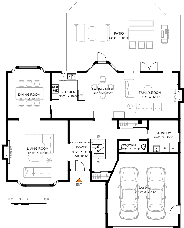
MAIN FLOOR 1,453 SQ.FT. CH: 8'-0"
