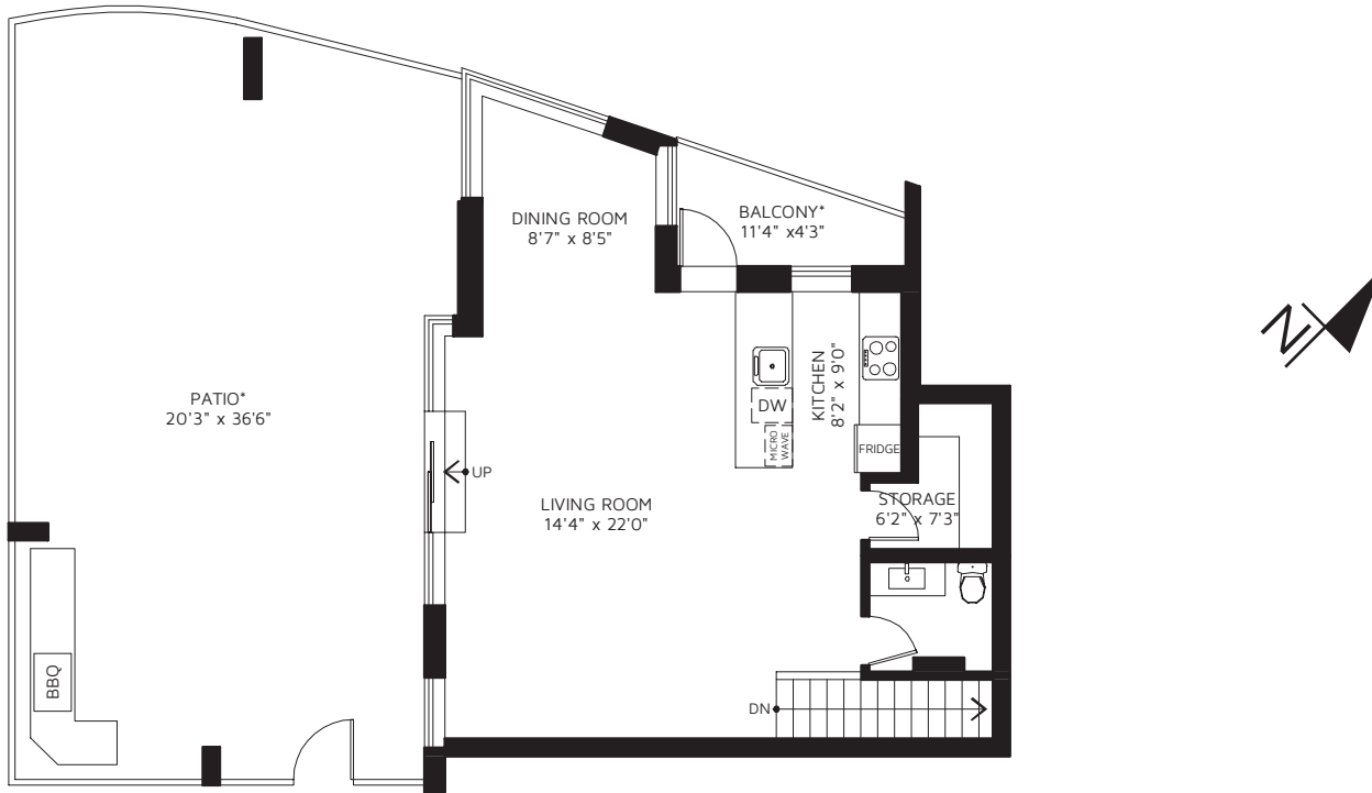
UPPER FLOOR
