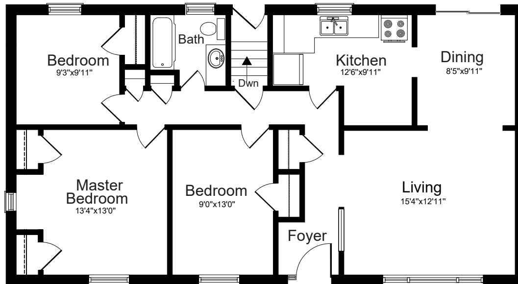
MAIN FLOOR 1180 sq ft
