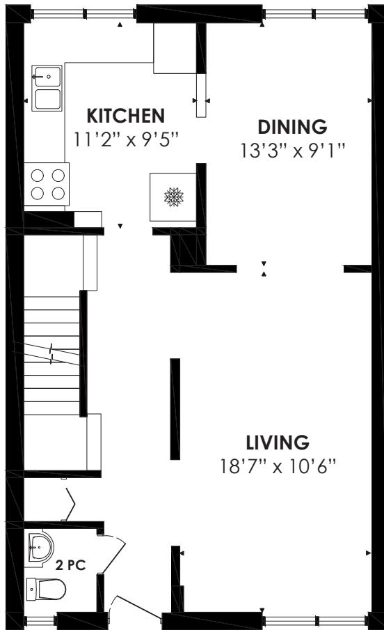
MAIN FLOOR 725 SQ FT
