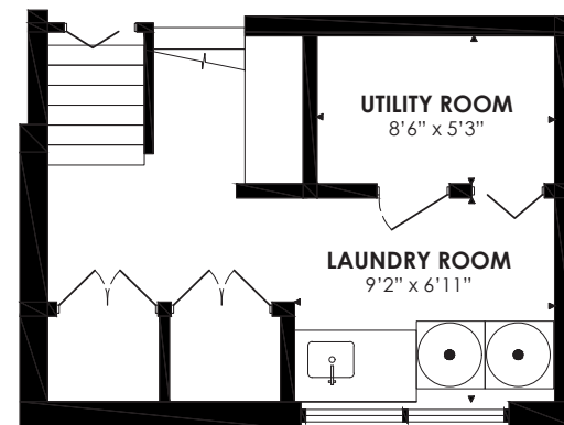
LOWER FLOOR 285 sq. ft.
