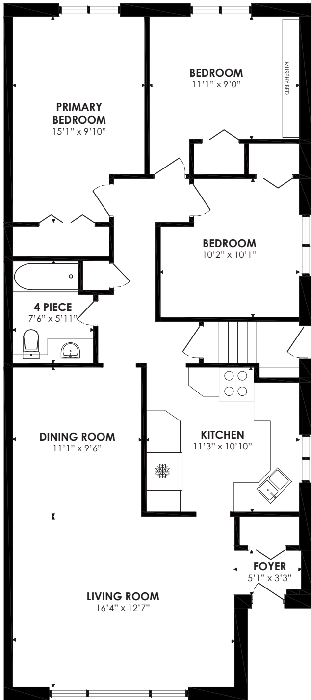
MAIN LEVEL 1155 sq. ft.
