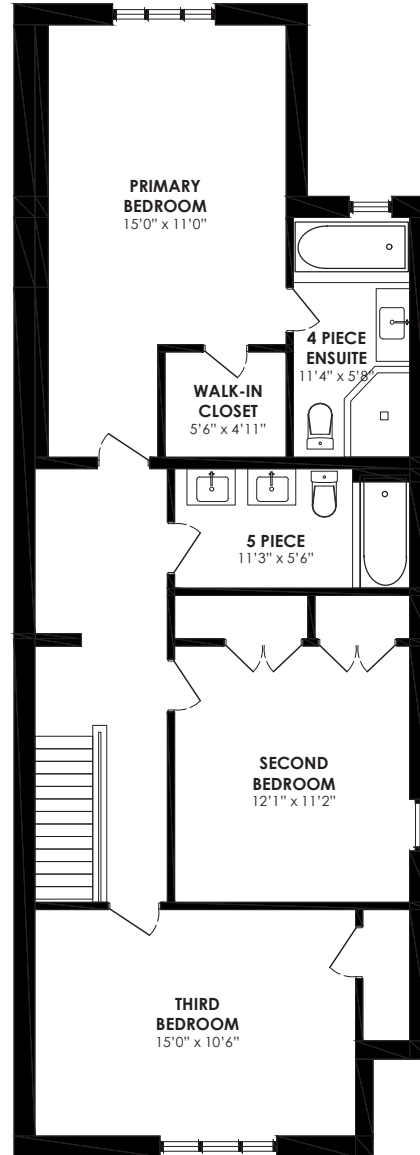
SECOND LEVEL 995 sq. ft.
