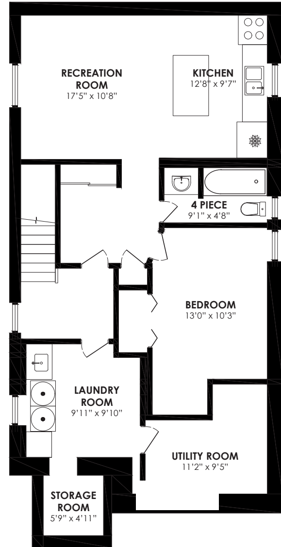
LOWER LEVEL 1070 sq. ft.
