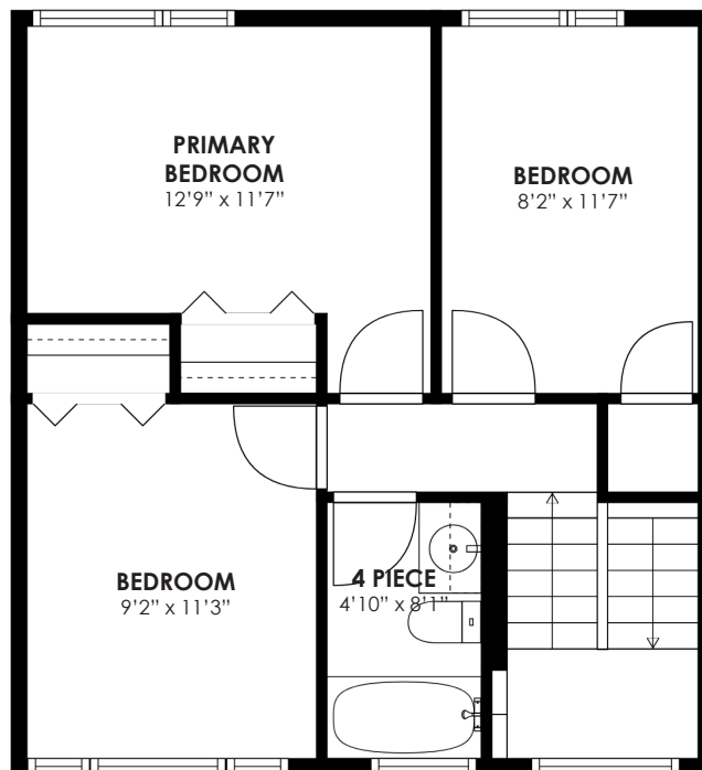
SECOND LEVEL 493 Sq. Ft.
