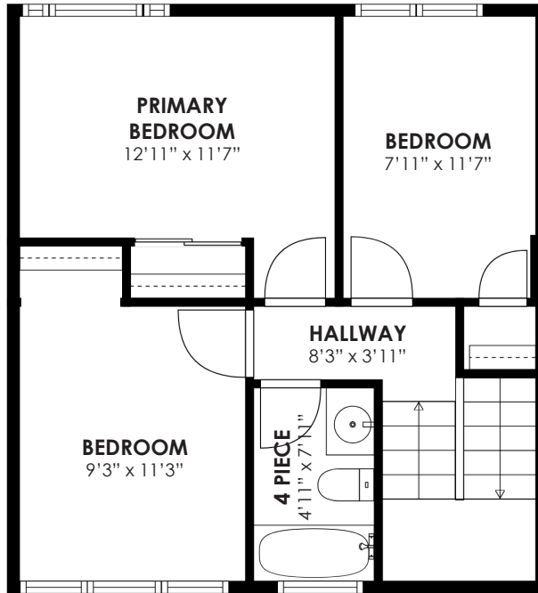
SECOND FLOOR 524 Sq. Ft.
