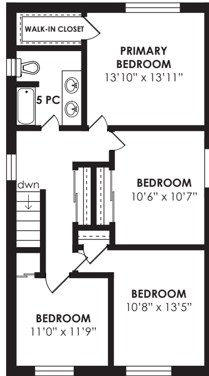
2ND FLOOR 1154 SQ FT
