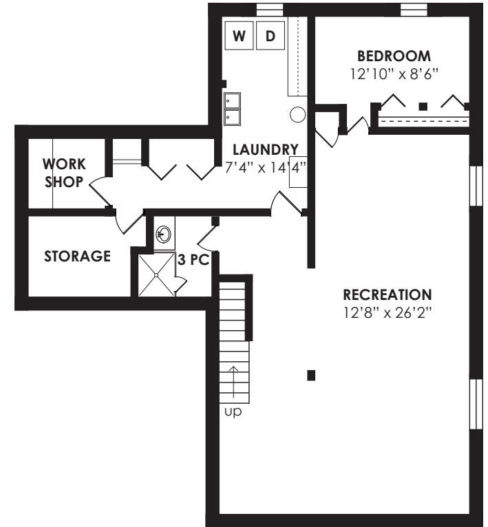
BASEMENT 1490 SQ FT
