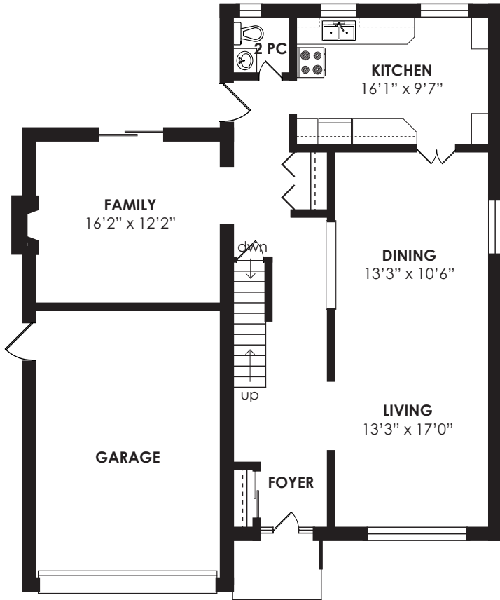
MAIN FLOOR 1490 SQ FT
