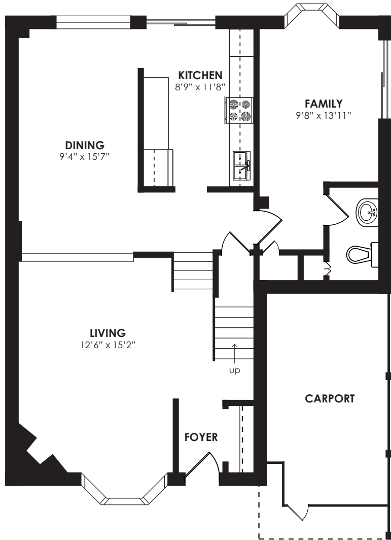
MAIN LEVEL 930 SQ FT
