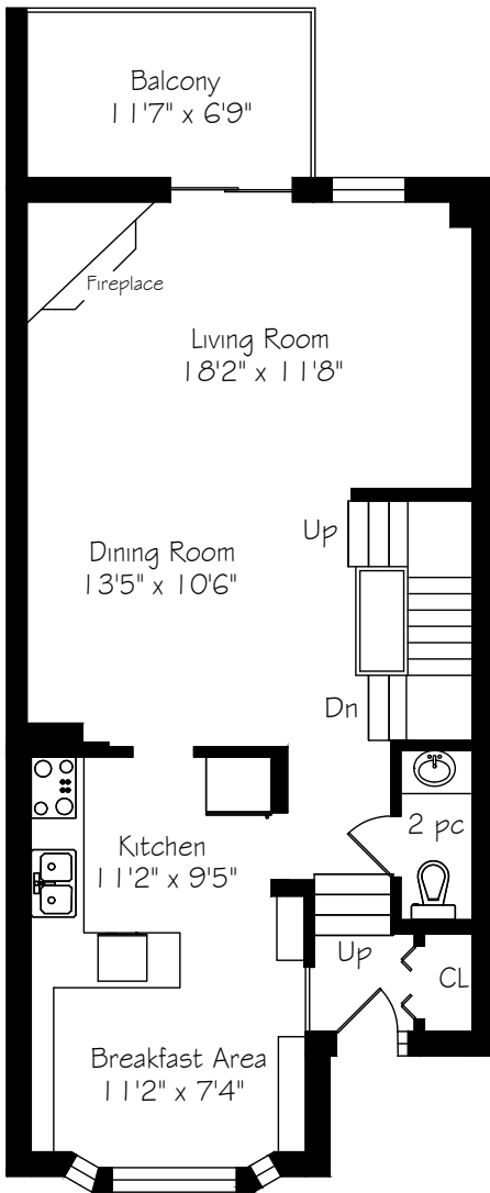
Main Floor 752 Square Feet
