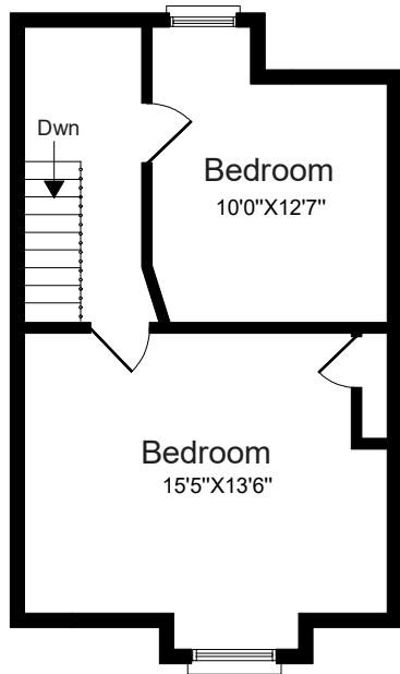
3RD FLOOR 435 sq ft
