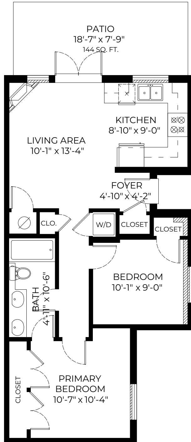
FLOOR PLAN Ceiling Height: 8'-0"
