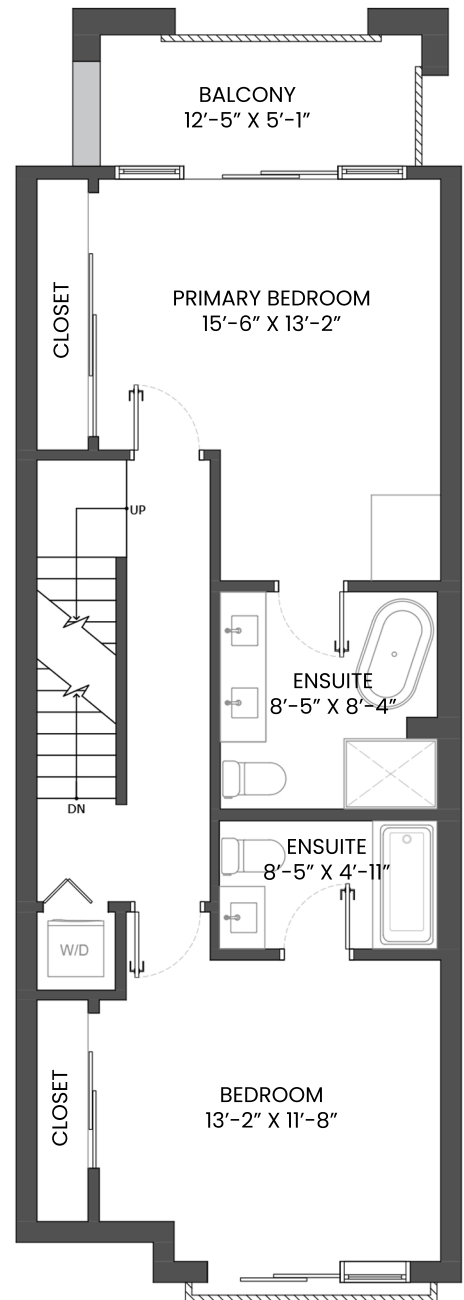
UPPER FLOOR PLAN Ceiling Height: 10'-0"
