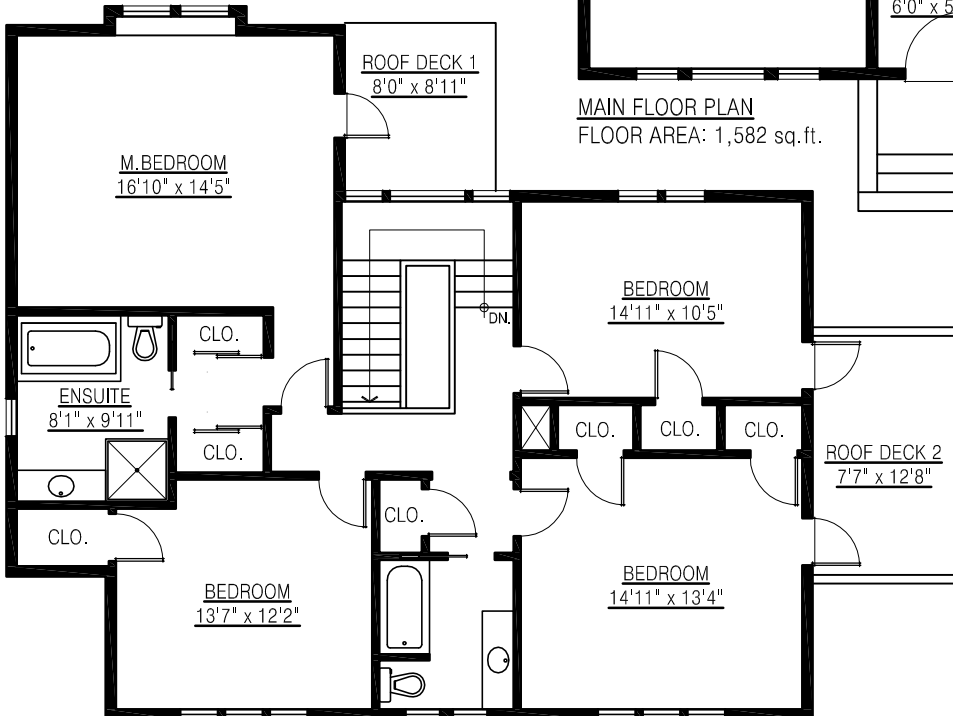
UPPER FLOOR PLAN FLOOR AREA: 1,314 sq.ft.
