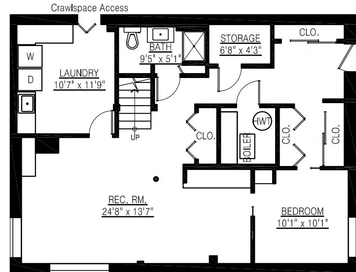
LOWER FLOOR PLAN FLOOR AREA: 1,037 sq.ft.
