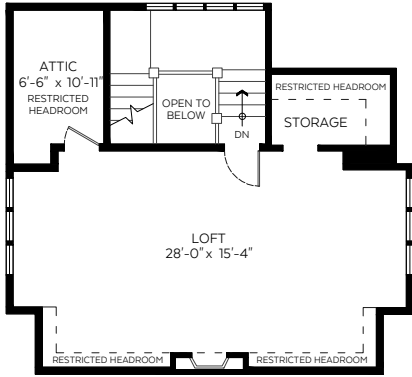
Top Floor Plan Floor Area: 523 sq.ft. Ceiling Height: 8 ft.
