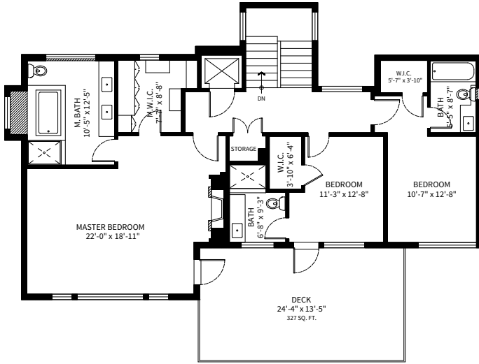
UPPER FLOOR PLAN Ceiling Height: 8'-0"
