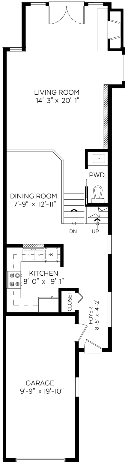
Main Floor Plan Floor Area: 686 sq.ft.
