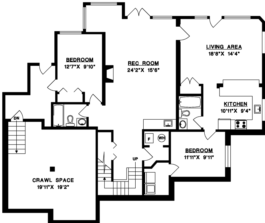
LOWER FLOOR
