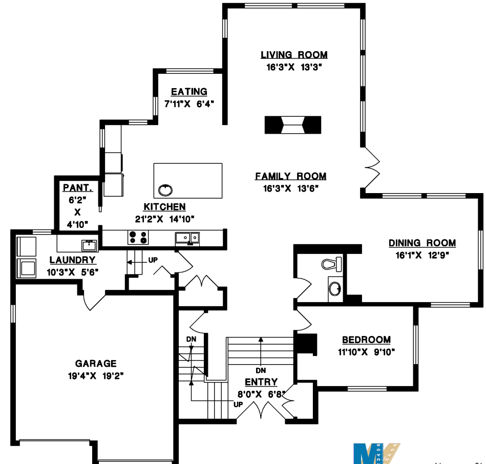
MAIN FLOOR
