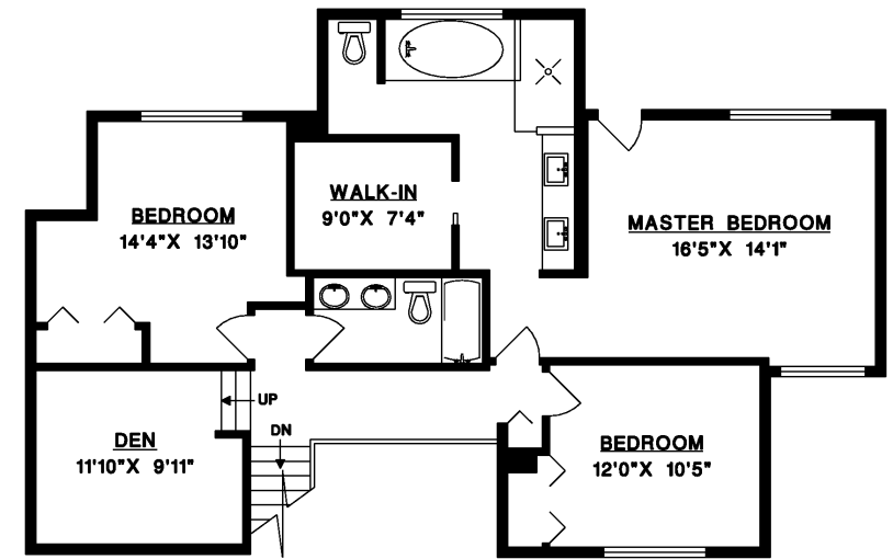
UPPER FLOOR
