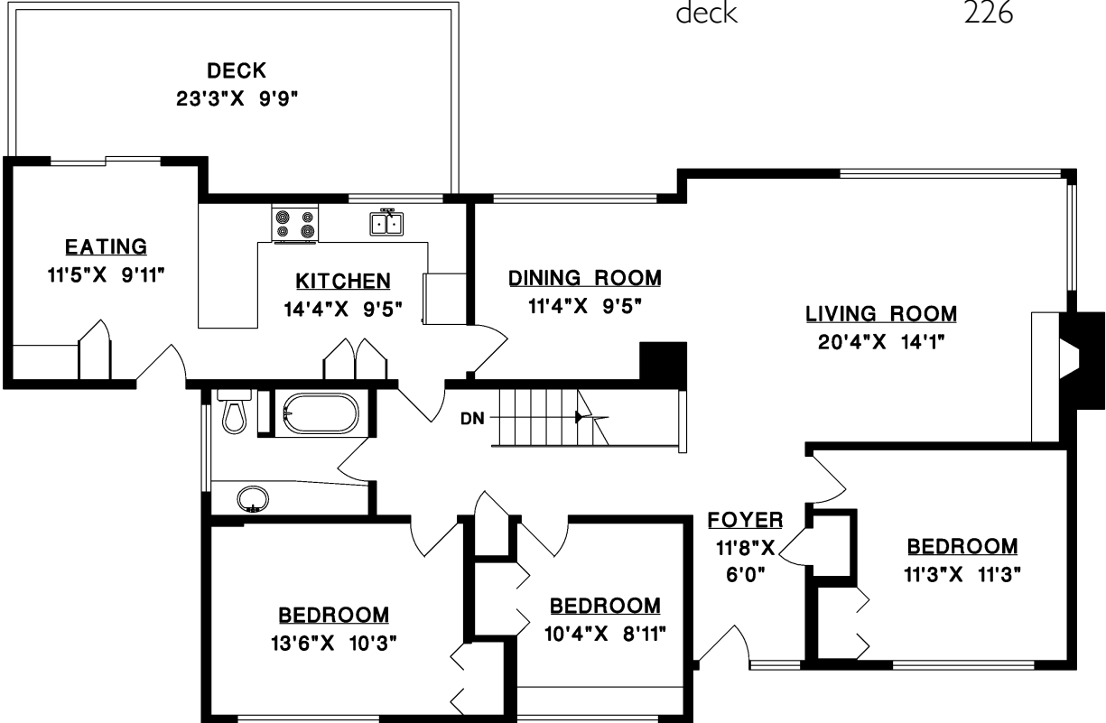
MAIN FLOOR
