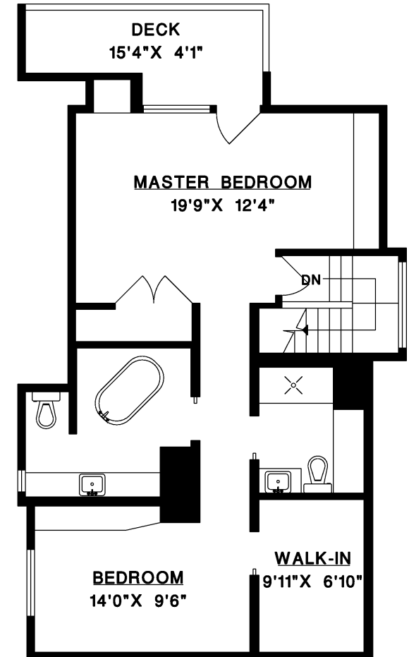
UPPER FLOOR
