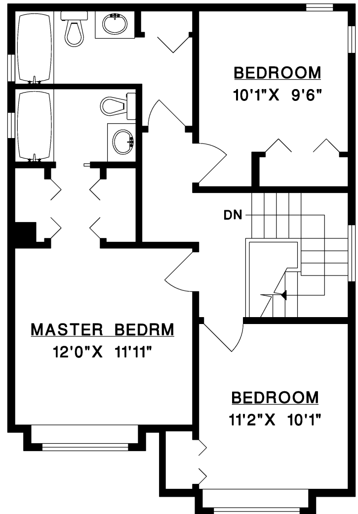
UPPER FLOOR
