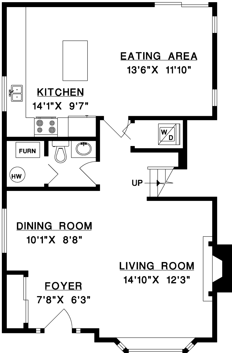
MAIN FLOOR
