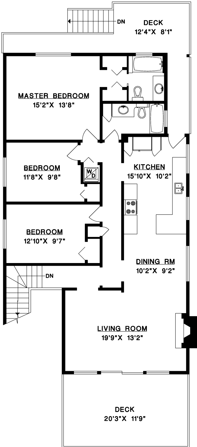
MAIN FLOOR
