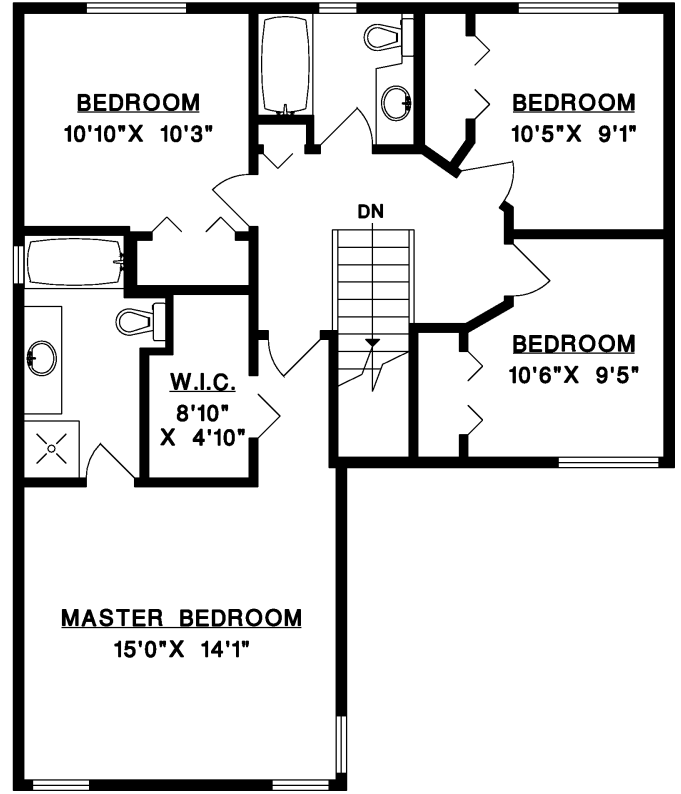
UPPER FLOOR
