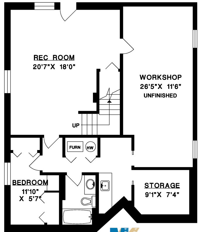
LOWER FLOOR
