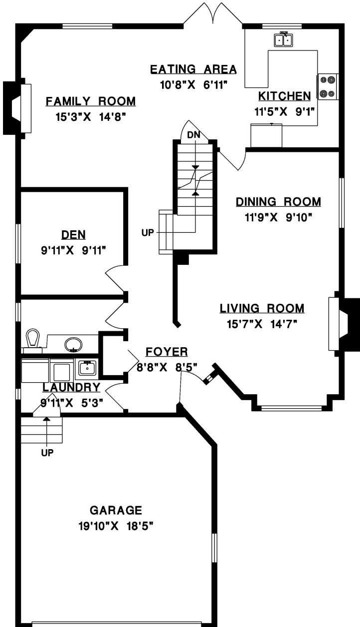
MAIN FLOOR
