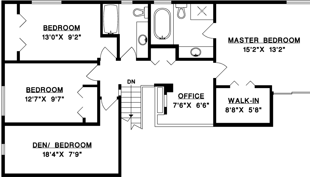
UPPER FLOOR
