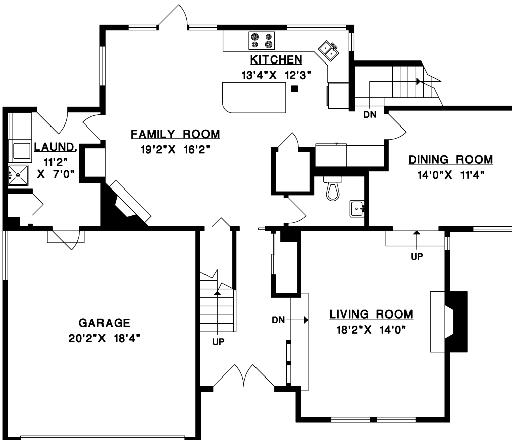
MAIN FLOOR
