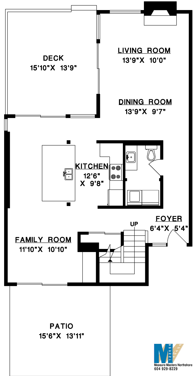
MAIN FLOOR
