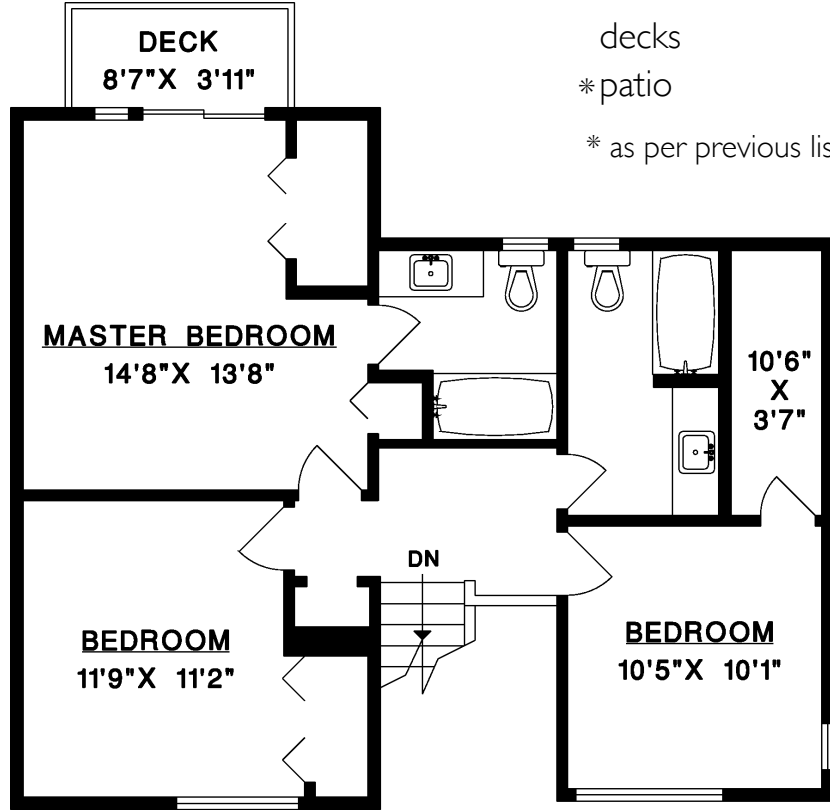
UPPER FLOOR
