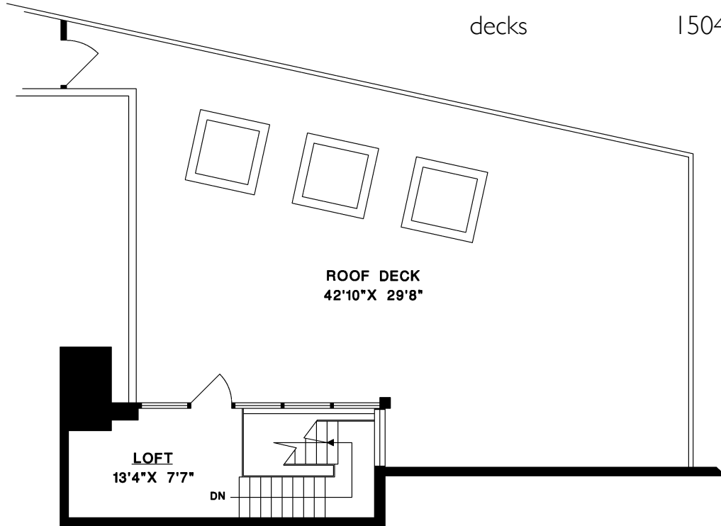
UPPER FLOOR
