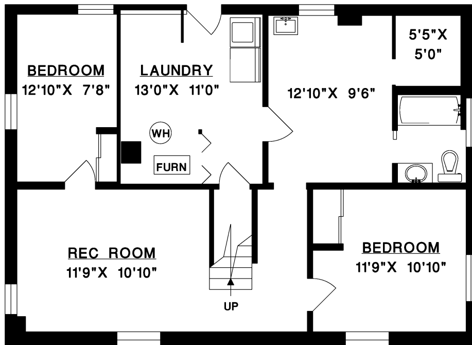
LOWER FLOOR
