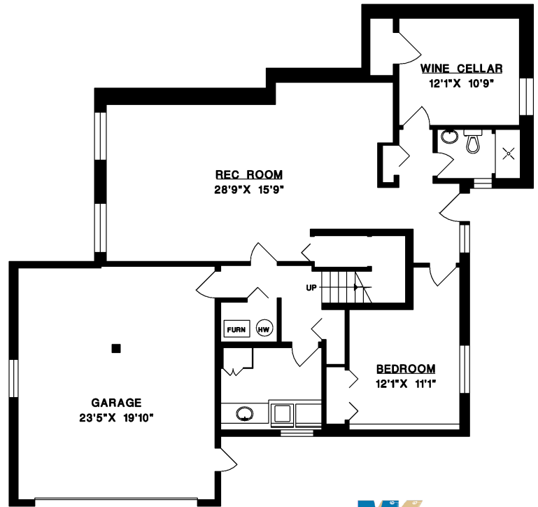
LOWER FLOOR
