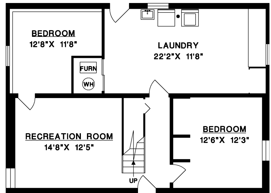
LOWER FLOOR
