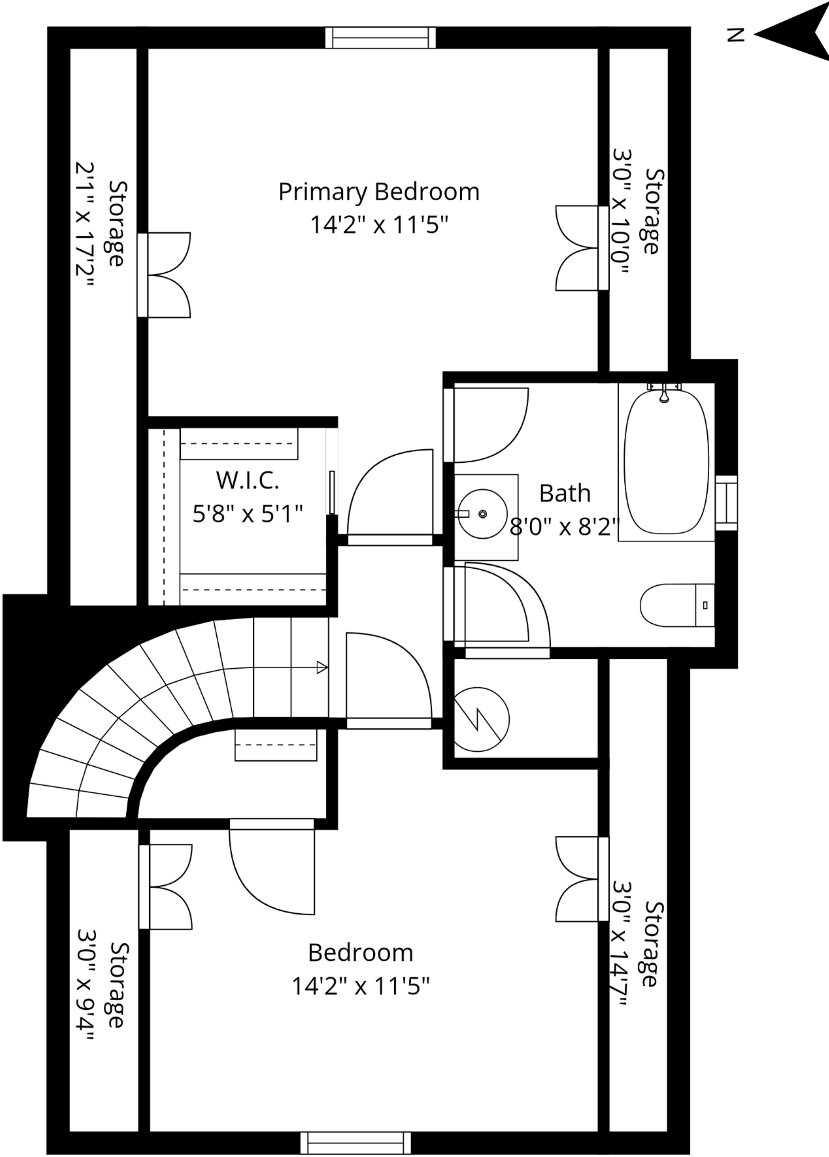
Upper Level - 567 Sq.Ft
