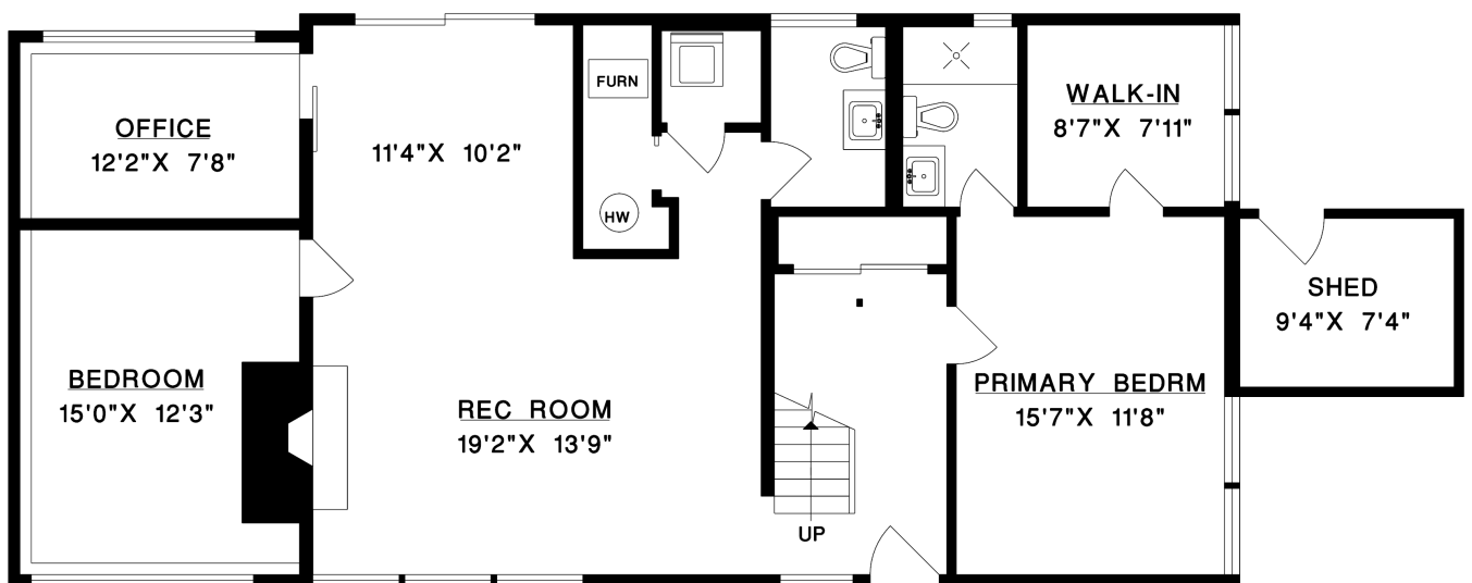
LOWER FLOOR
