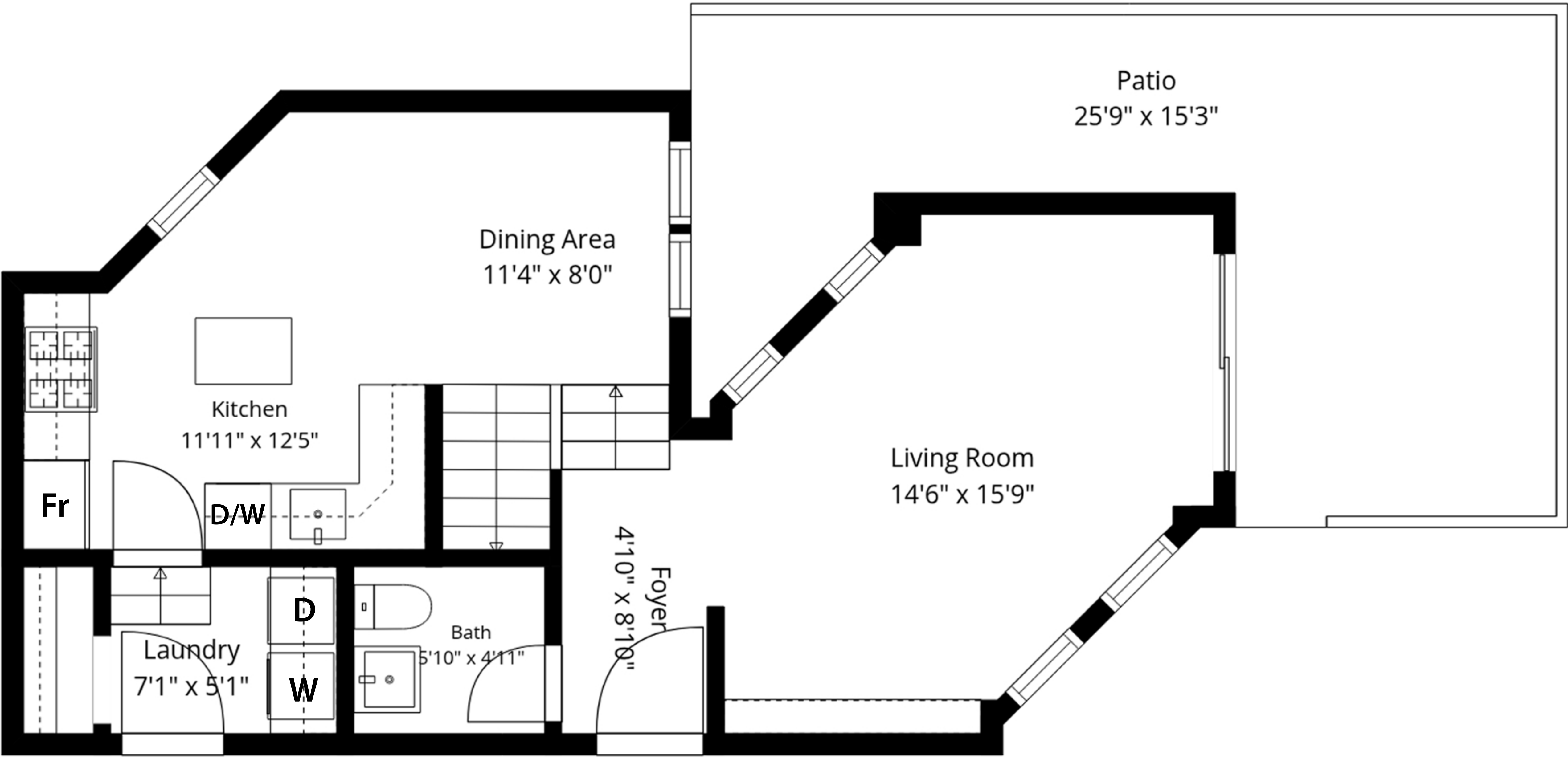
Main Level - 602 Sq.Ft Ceiling Height - 8'0" - 10'3"
